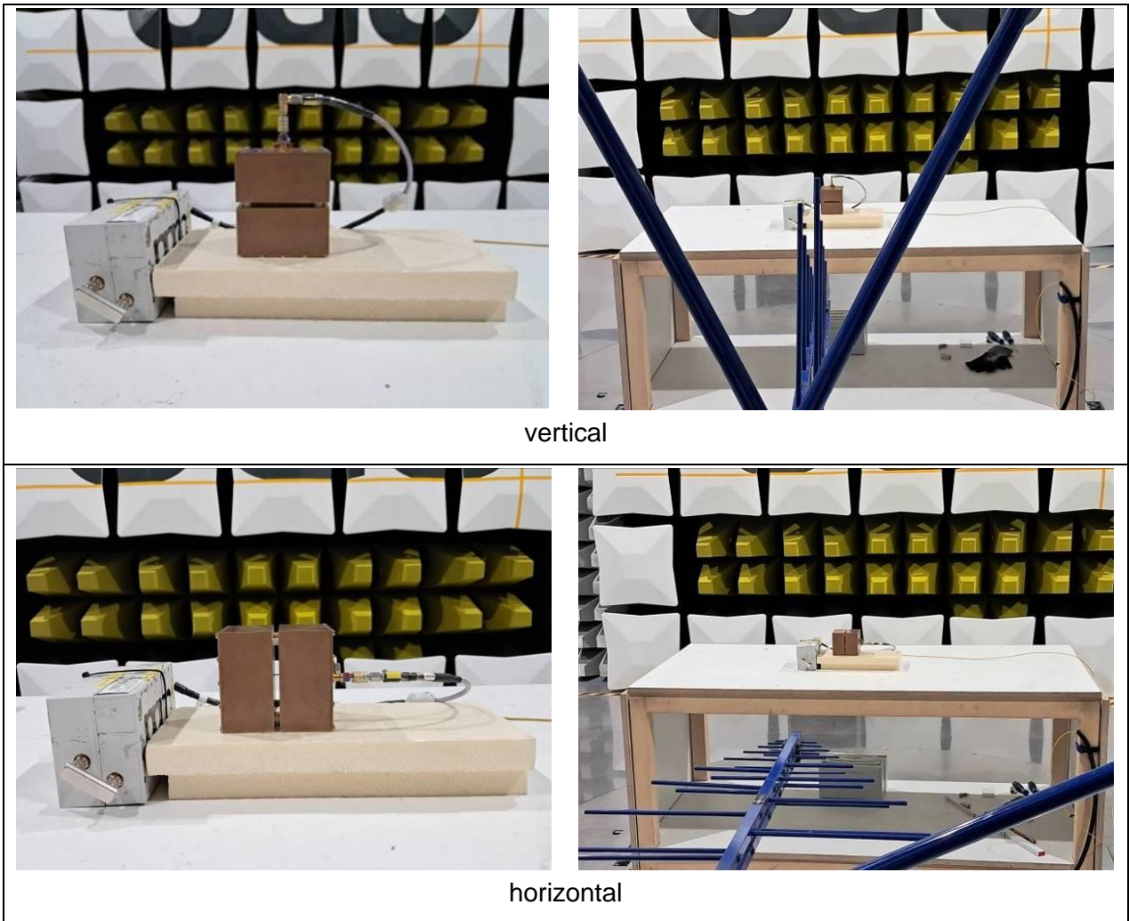
Figure 6-6: test setup reference measurements for position front/top
