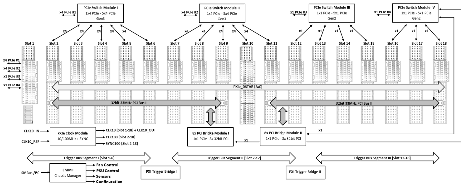
Figure 3: Backplane Topology
