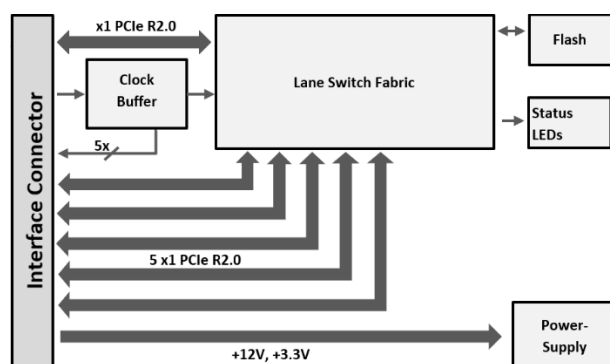
Figure 5: PCIe 6 Lane Switch Module Gen2
