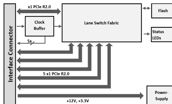
Figure 5: PCIe 6 Lane Switch Module
