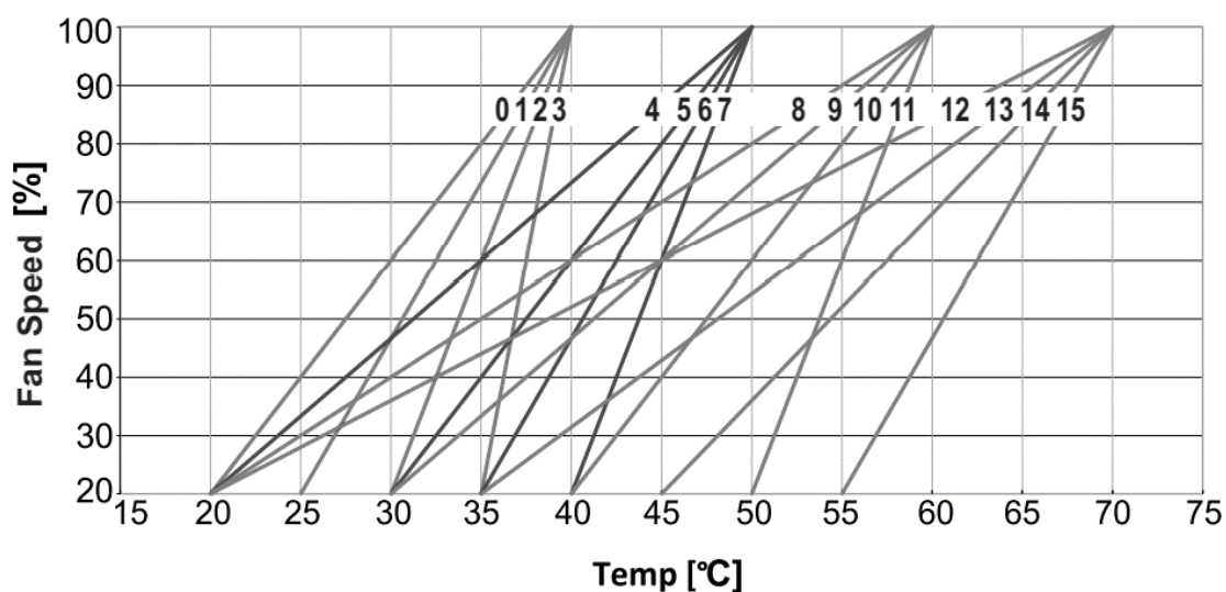
Figure 15: Fan Curves
