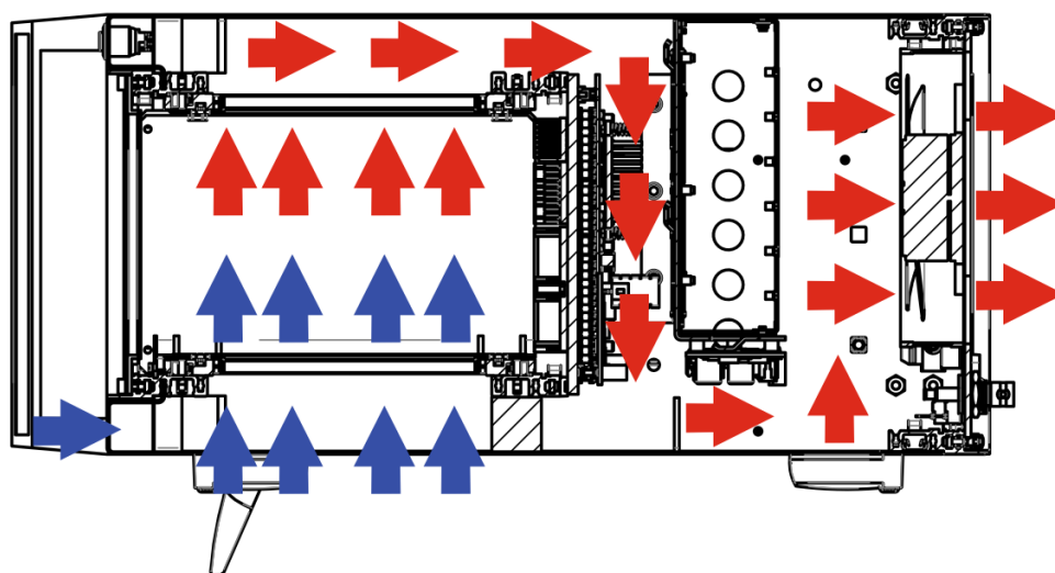
Figure 11: Air Flow
