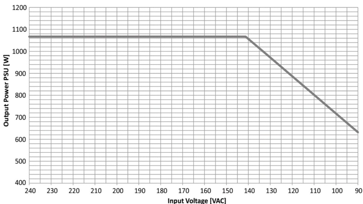
Figure 10: Output Power Derating
