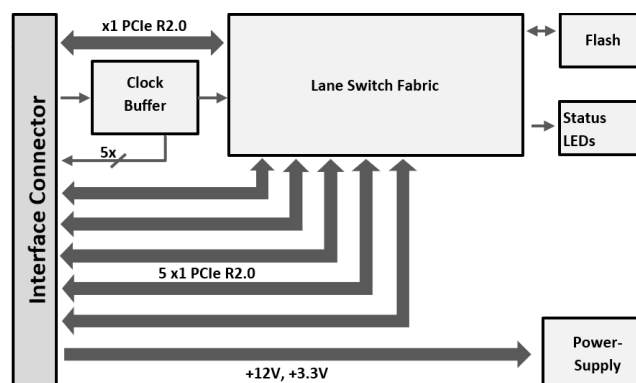
Figure 5: PCIe 6 Lane Switch Module Gen2
