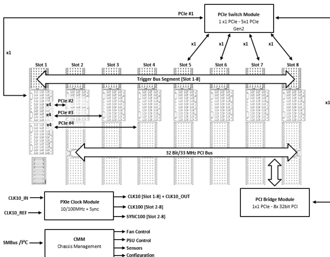
Figure 3: Backplane Topology
