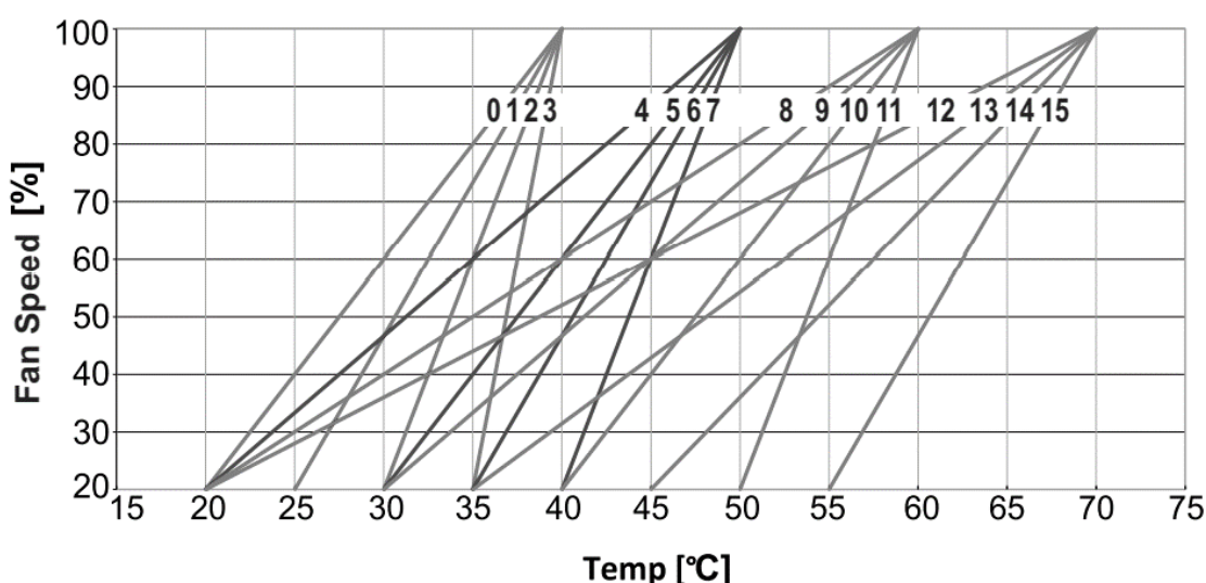
Figure 15: Fan Curves
