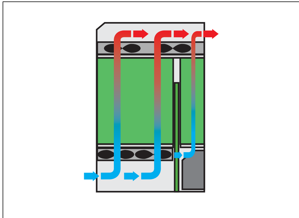
Figure 18: System Airflow Path
