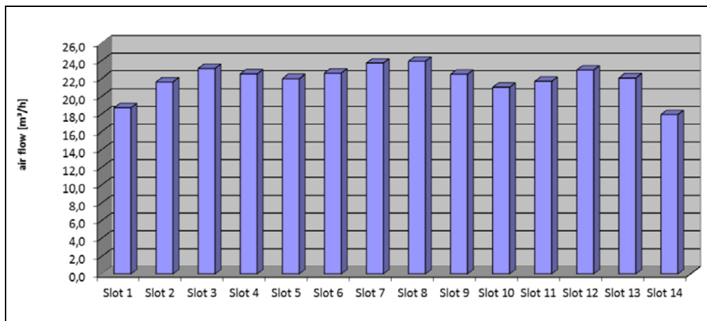
Figure 23: Rear Board Air Distribution 11990-190
