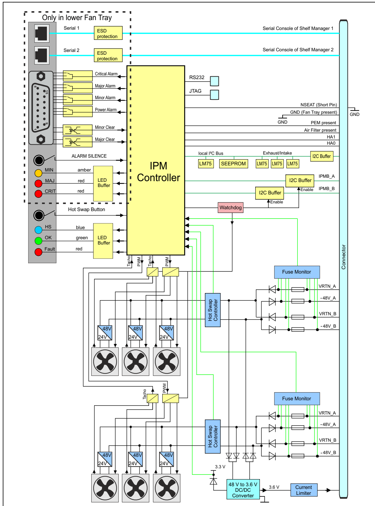
Figure 14: Fan Tray Block Diagram
