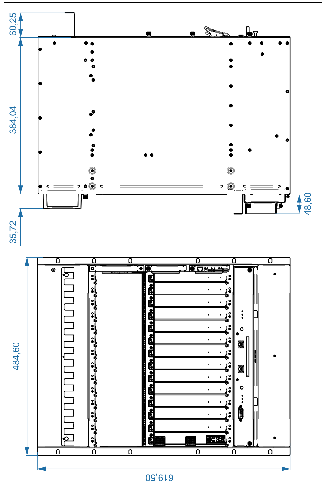
Figure 39: Shelf dimensions
