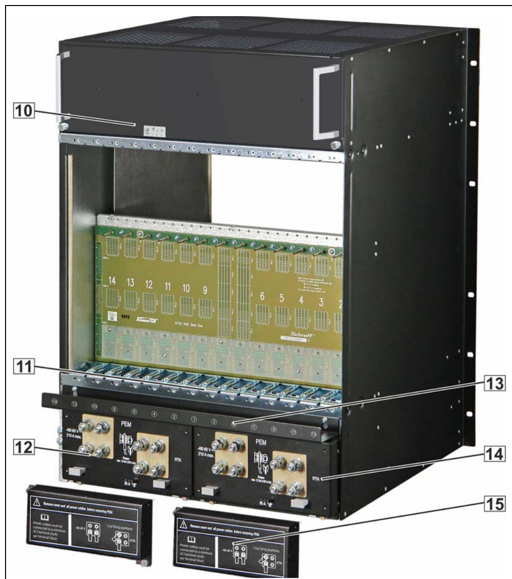
Figure 2: 11990-190 Shelf Rear View
