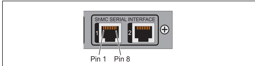
Figure 16: RS-232 Serial Console Interfaces
