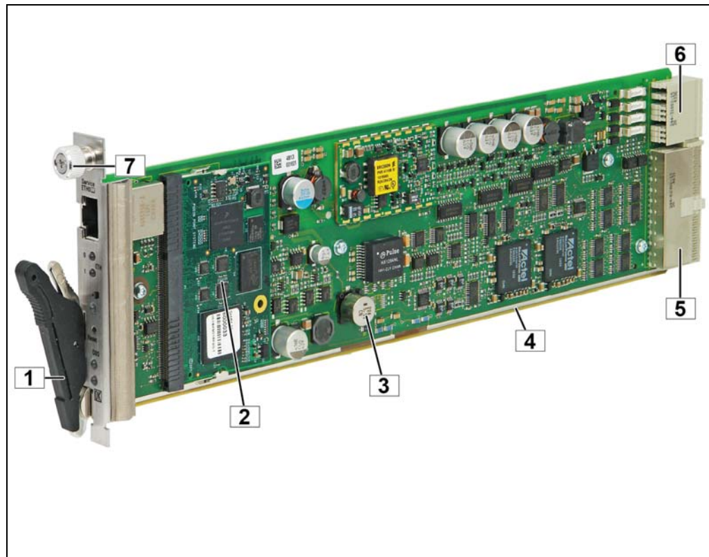
Figure 33: Schroff Shelf Manager
