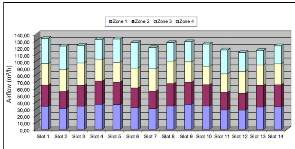
Figure 21: Front Board Air Distribution 11990-192
