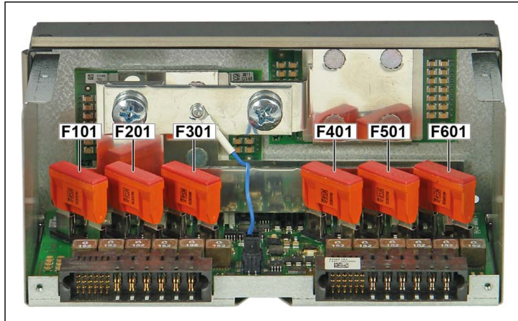
Figure 31: PEM Fuses
