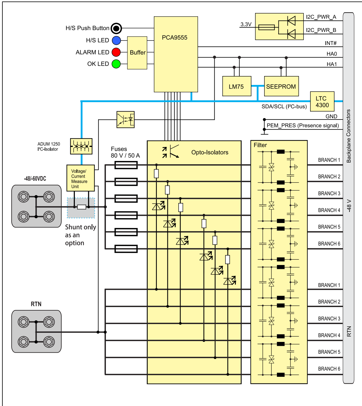
Figure 30: PEM Block Diagram
