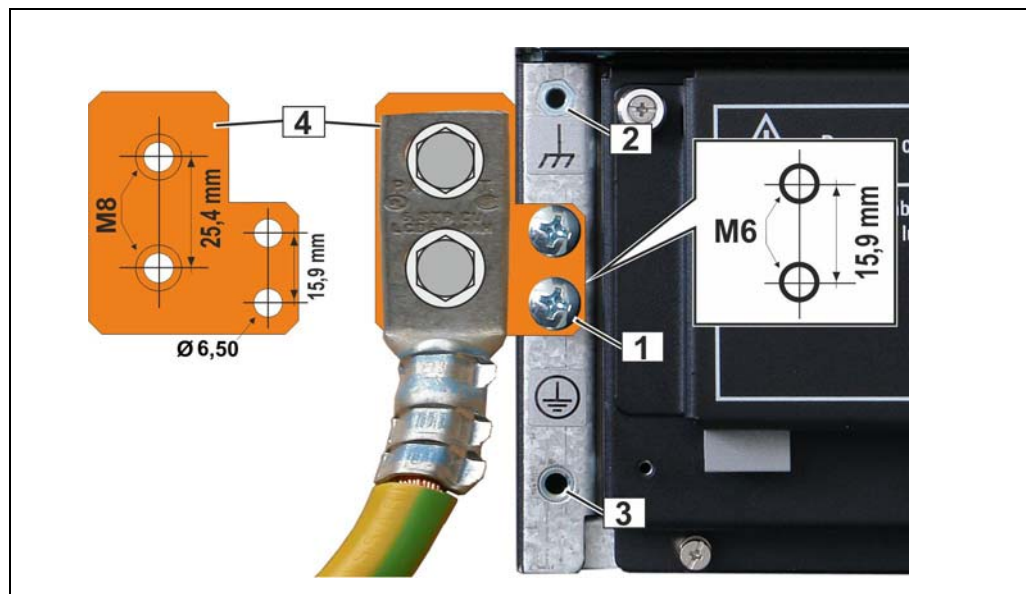
Figure 10: Shelf ground terminal with adapter kit
