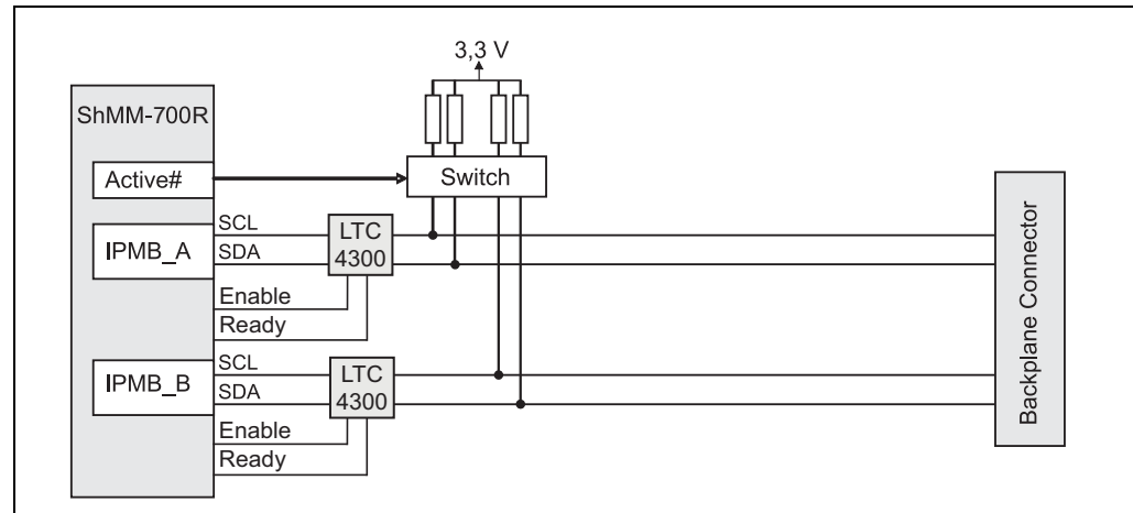
Figure 35: Block diagram bused IPMB
