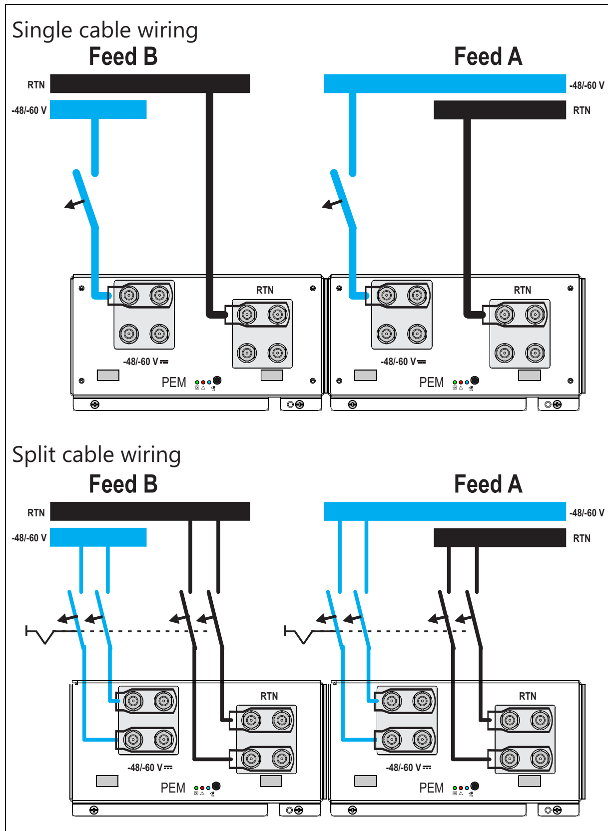
Figure 28: PEM Wiring
