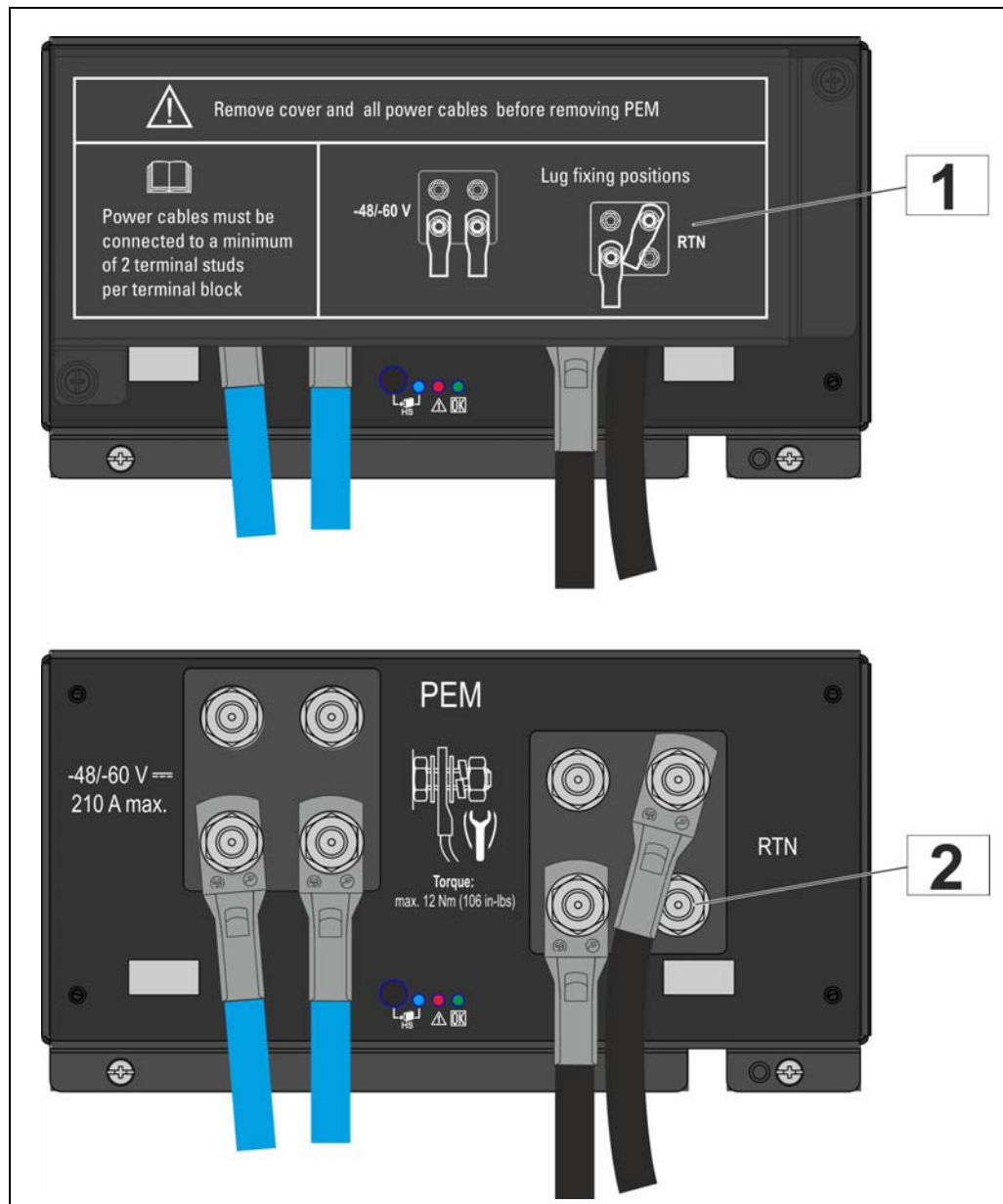
Figure 27: PEM Front View
