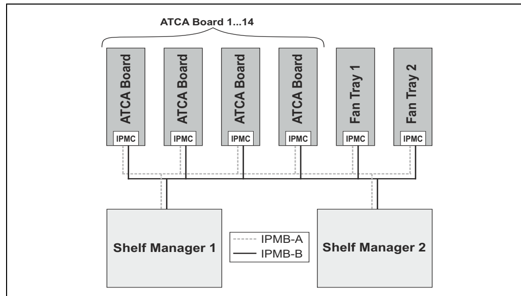
Figure 5: Bused IPMB
