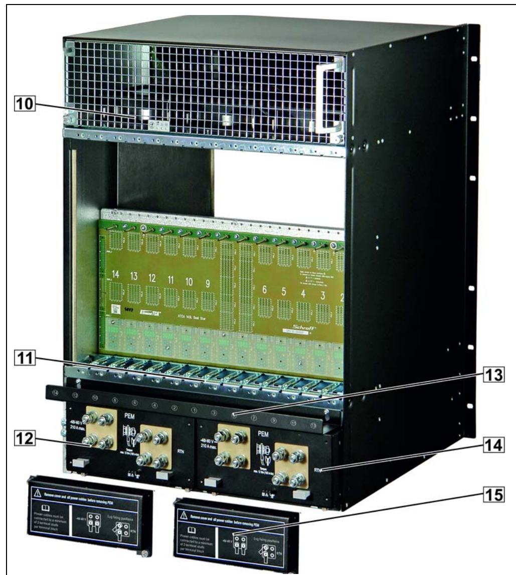
Figure 4: 11990-192 Shelf Rear View
