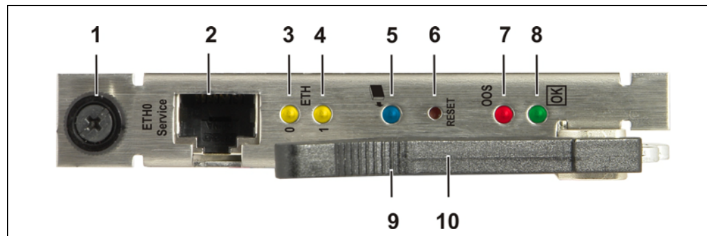
Figure 34: Shelf Manager Front Panel Components
