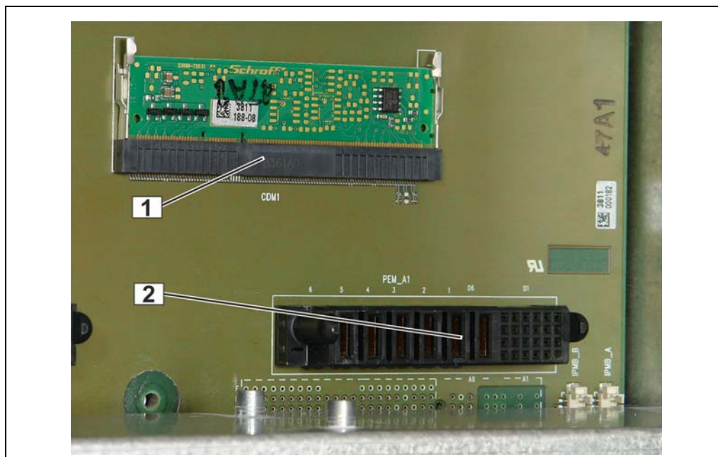
Figure 6: Chassis Data Module 1 (CDM 1)
