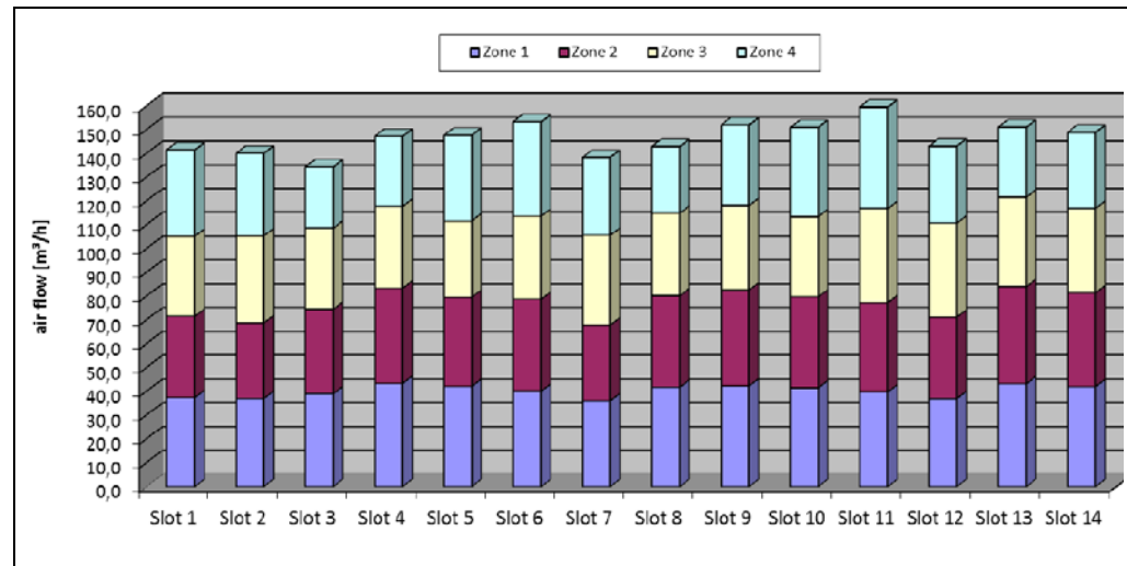
Figure 19: Front Board Air Distribution 11990-190
