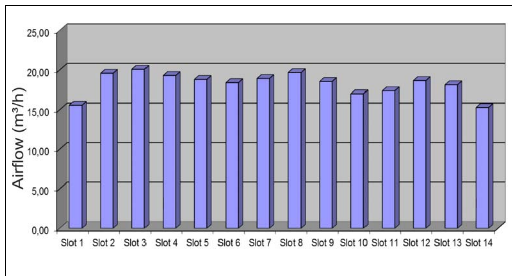
Figure 25: Rear Board Air Distribution 11990-192
