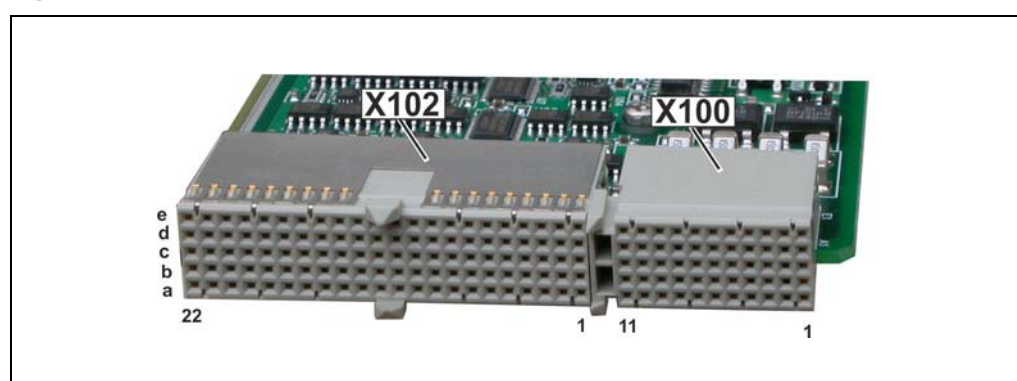
Figure 38: Backplane Connectors
