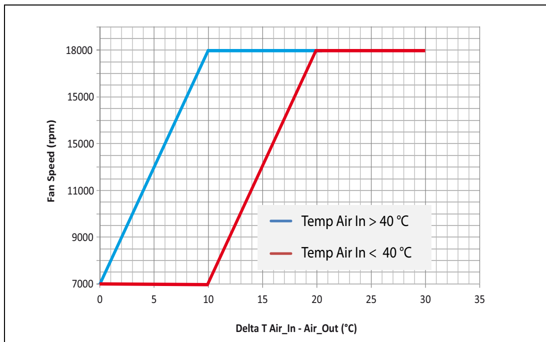
Figure 5: Fan Speed vs Temperature
