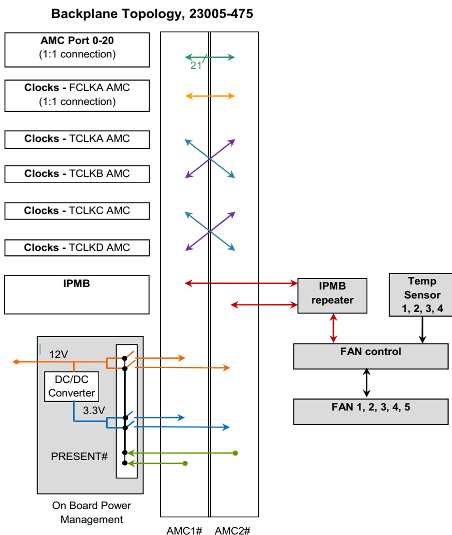
Figure 2: Backplane Topology
