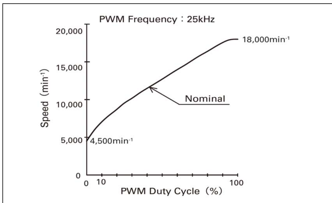
Figure 6: PWM vs Fan Speed
