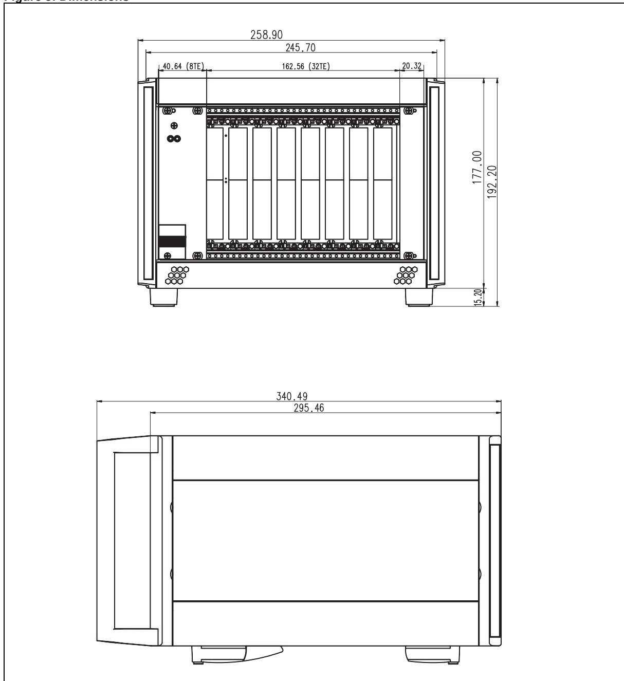
Figure 5: Dimensions
