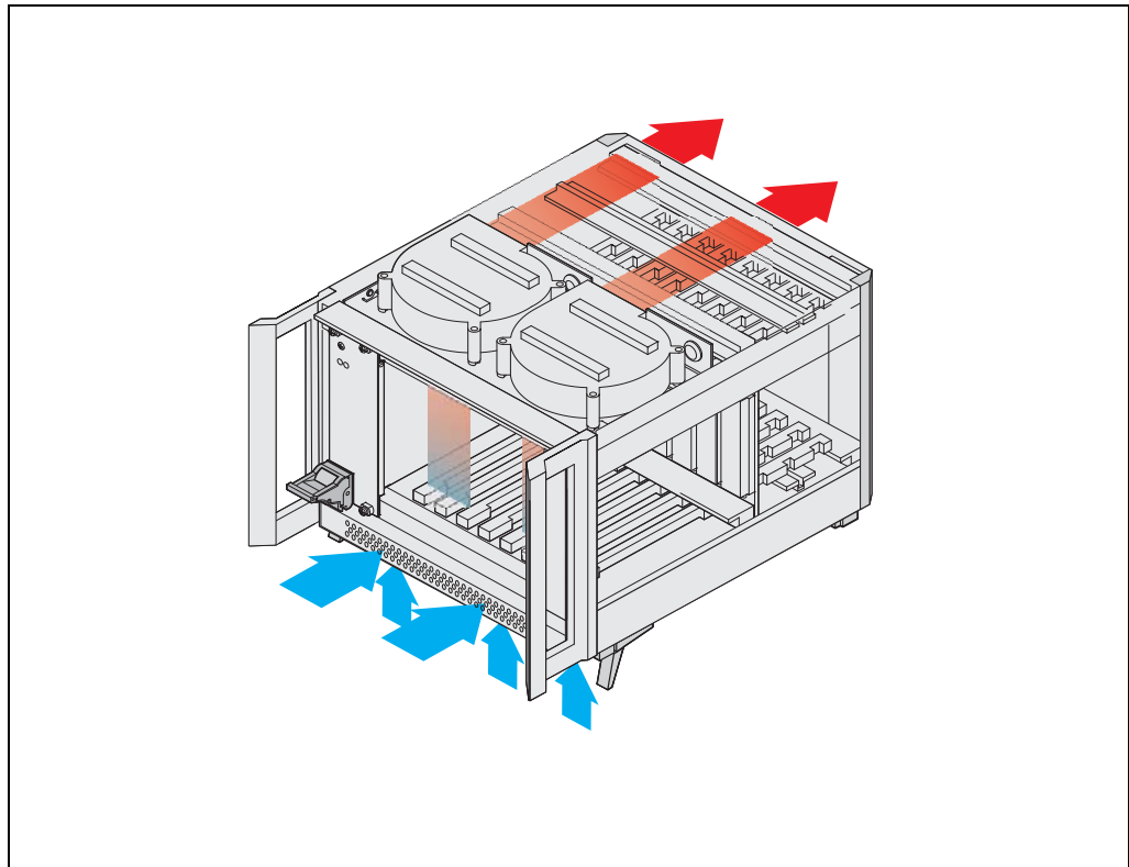
Figure 4: Airflow
