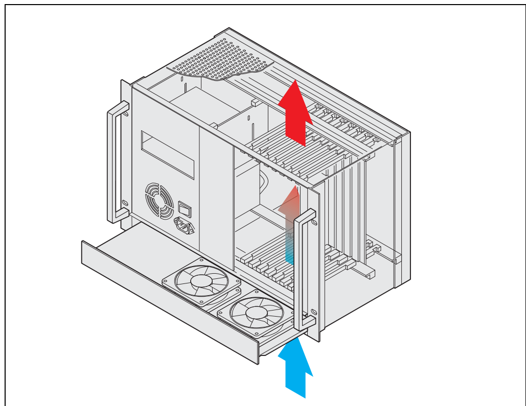
Figure 2: Airflow
