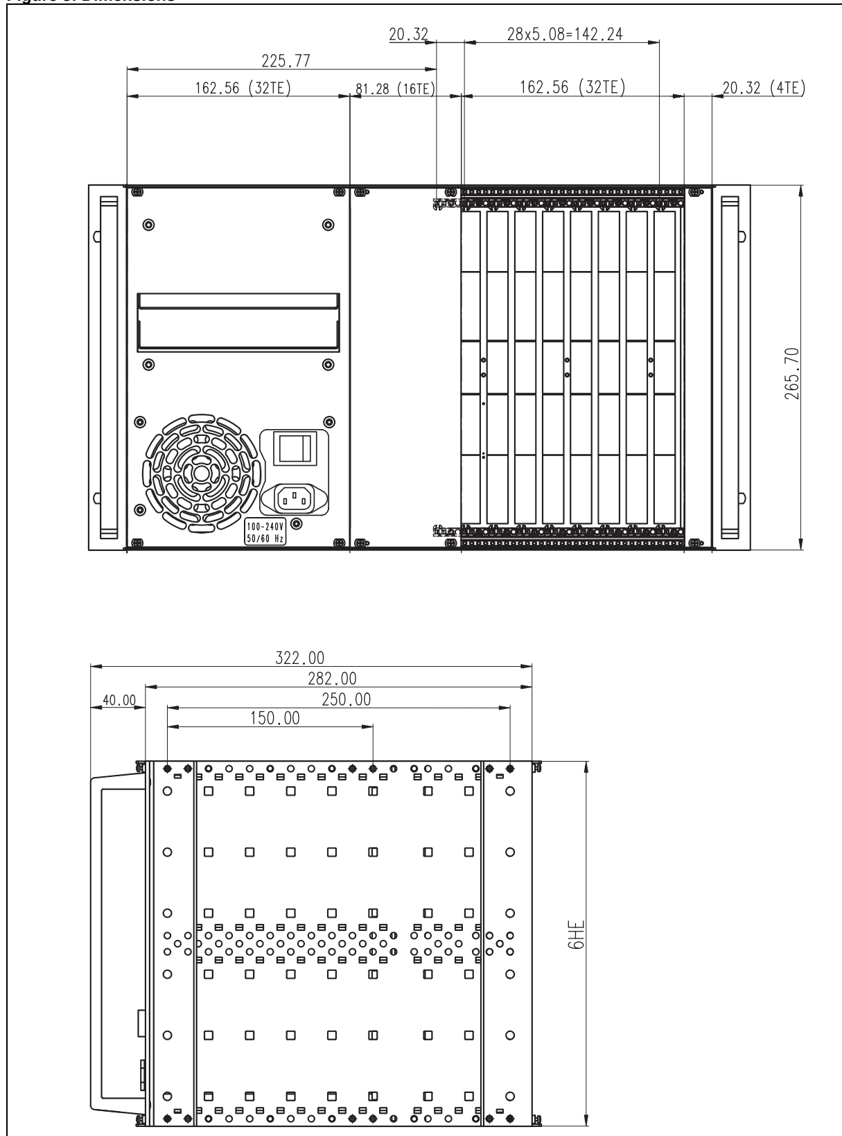
Figure 3: Dimensions
