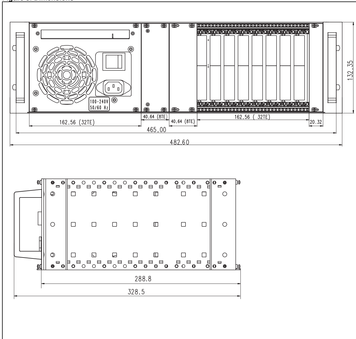
Figure 3: Dimensions
