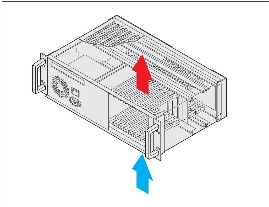
Figure 2: Airflow
