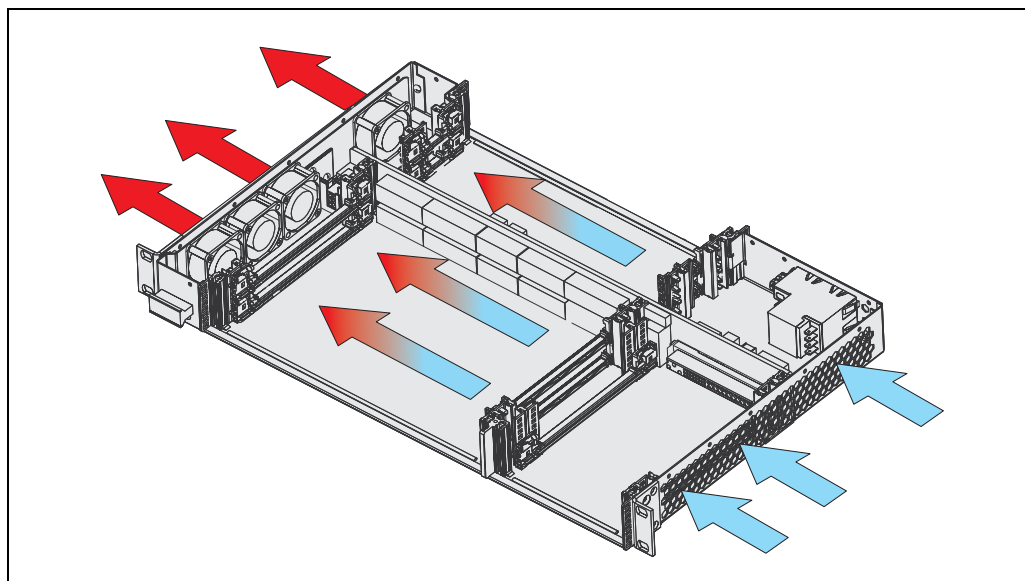
Figure 5: Airflow
