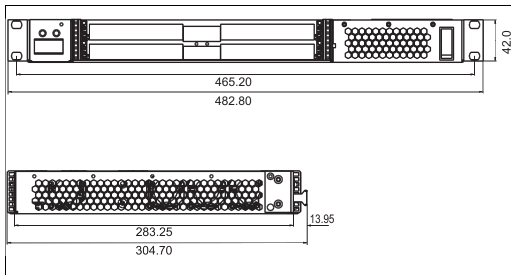
Figure 6: Dimensions
