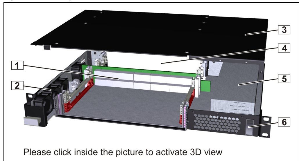
Figure 1: Subrack System Overview
