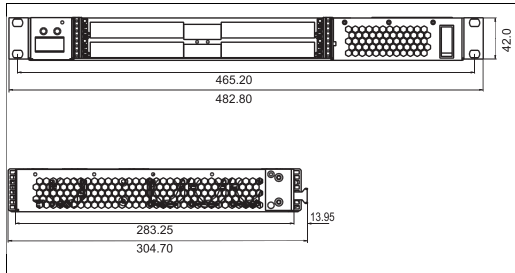
Figure 5: Dimensions
