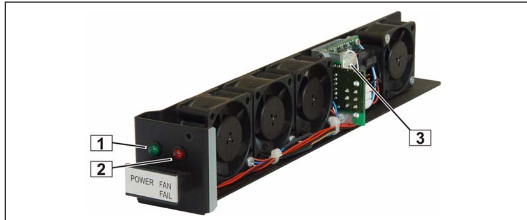
Figure 4: Fan Tray
