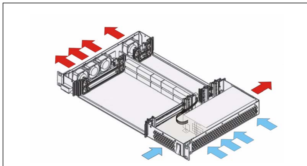
Figure 5: Airflow
