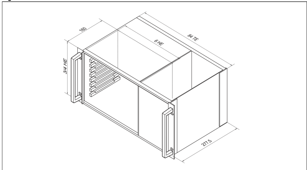
Figure 7: Dimensions
