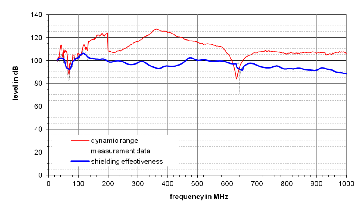
Fig. 7: Measurement results for direct radiation on LEFT-side of the EUT
