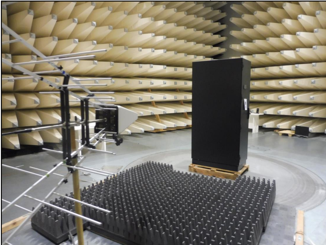
Photo 5: radiated immunity
